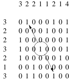
Fig. 1. A binary matrix having period (2, 3) . The integers at the beginning of each row and column correspond to its horizontal and vertical projections, respectively. The circled entry 1 is linked, by periodicity, with the two pointed ones.
